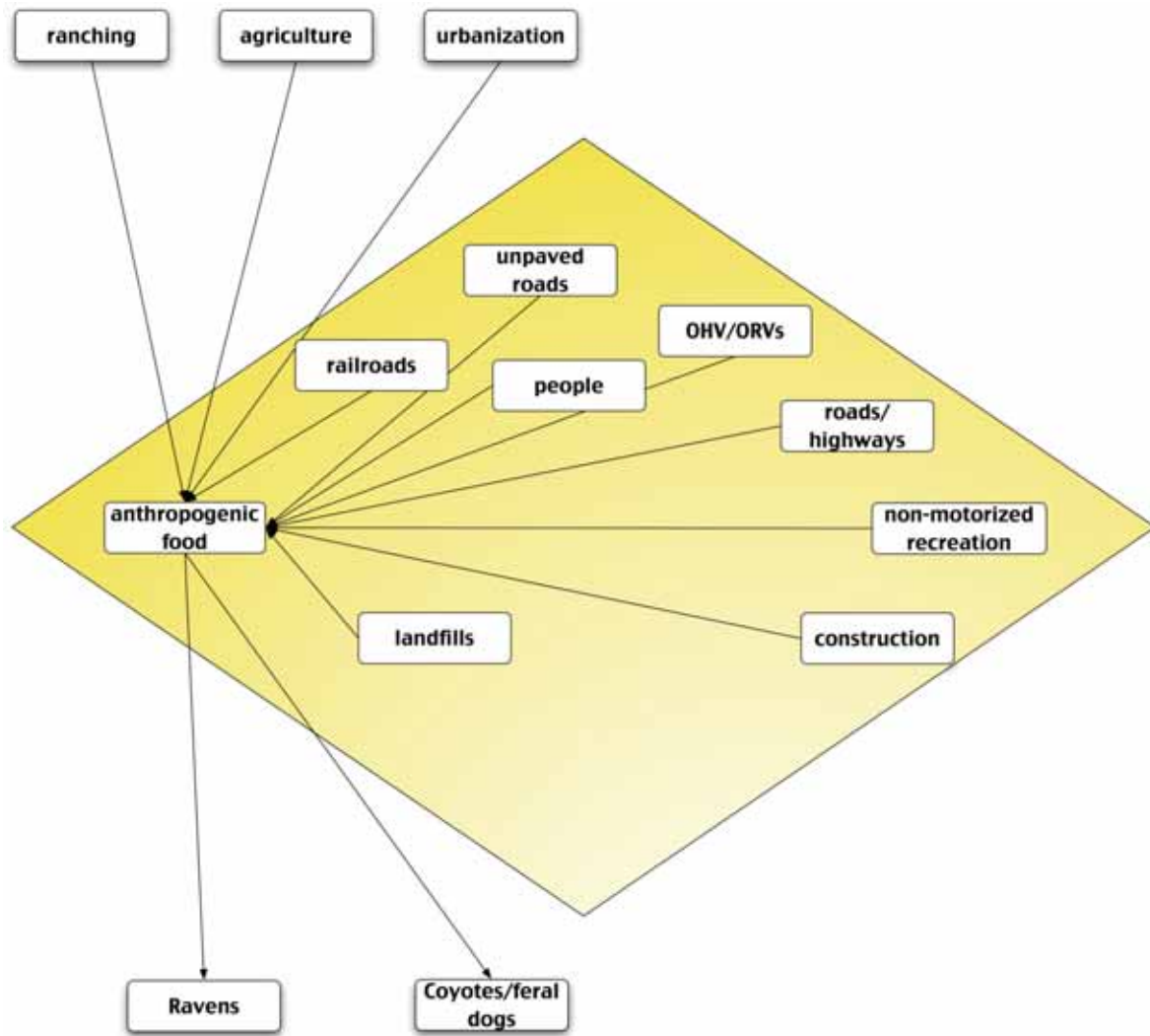
Fig. 5.2 A section from the Threats Network from Fig. 5.1 that shows how multiple land uses and human activities provide food subsidies to predators on tortoises, thereby increasing mortality.
